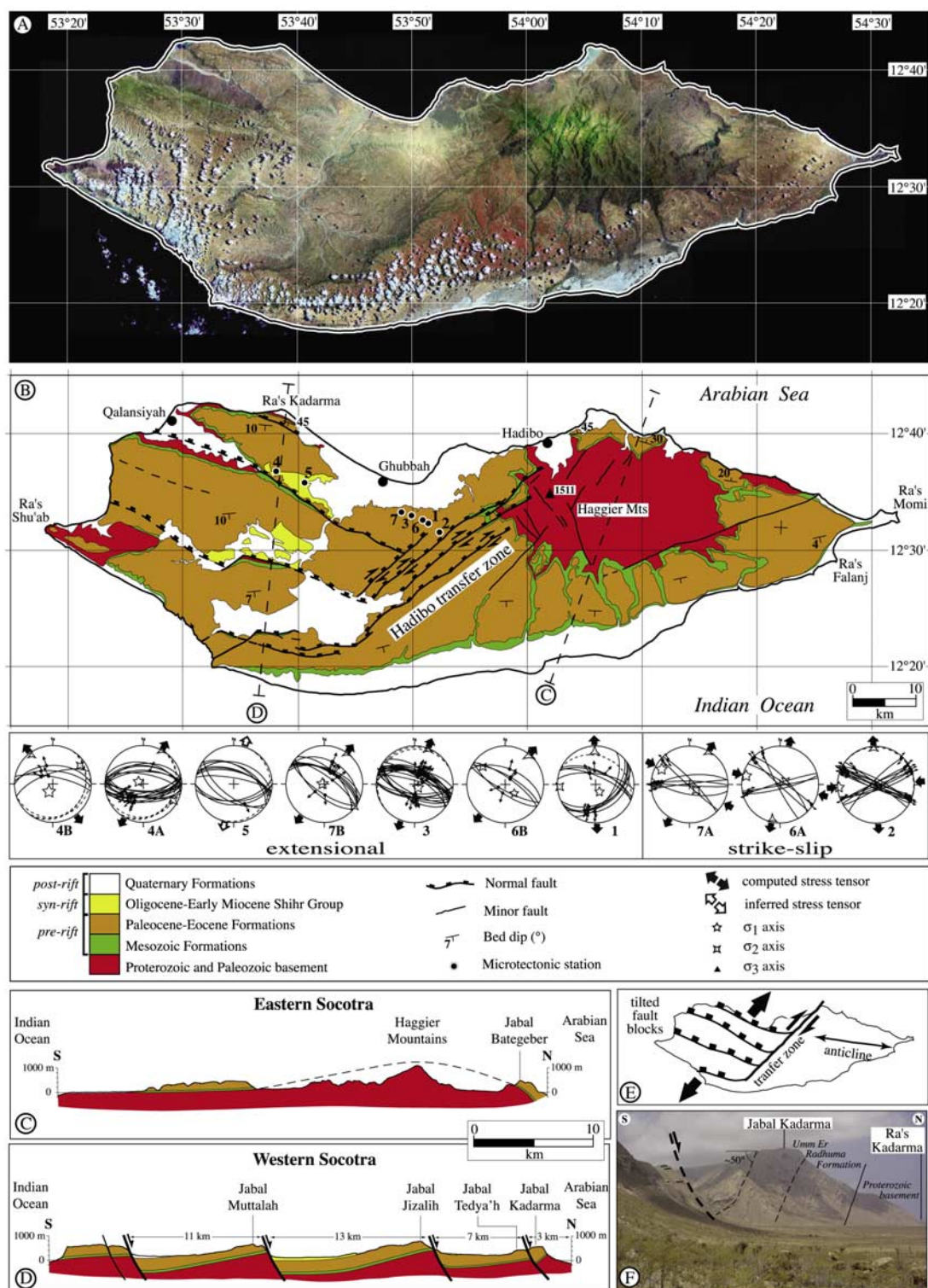
Figure 2. (a) Landsat image and (b) structural map of Socotra (after Landsat imagery and SRTM data interpretation, and Ministry of Oil and Minerals Resources [1990]) with stress field recorded in Tertiary formations. Stars in stereonets (equal-area lower hemisphere projection) correspond to the principal stress axes: \sigma_1 (five branches), \sigma_2 (four branches), and \sigma_3 (three branches). Arrows show the trend of the horizontal principal stresses computed from fracture analysis. Dashed line is for the bedding plane. (c) Cross section of eastern Socotra (location in Figure 2b). (d) Cross section of western Socotra. (e) Simplified structural map of Socotra. (f) Southward tilted fault block in Ra's Kadarma. Basement is exposed to the north along the coast and capped by tilted Cretaceous and Eocene strata. The tilt block has undergone rotation of \sim 50^\circ about a horizontal \sim E–W axis.
