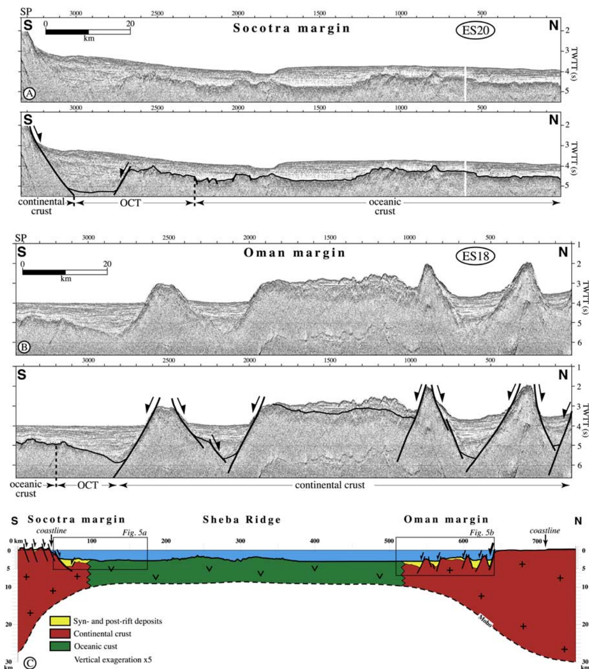
Figure 5. ES18 and ES20 seismic profiles off Oman and Socotra, respectively, from the Encens-Sheba cruise [d'Acremont, 2002], located in Figure 1. The ocean-continent transition (OCT) has been defined from joint analysis of seismic reflection, and free-air gravity and magnetic anomalies [d'Acremont et al. , 2005]. (a) Offshore Socotra, the continental margin is steep, narrow, and dominated by a northward shallow-dipping normal fault with a deep sedimentary basin at its toe. (b) The Oman margin displays horsts and grabens bounded by widely spaced conjugate faults with little block rotation. (c) Crustal cross section of the eastern Gulf of Aden combining the interpretations of seismic profiles ES18 and ES20, and the cross section of western Socotra in Figure 2d (location in Figure 1). The Moho geometry is speculative. SP are shotpoints.
