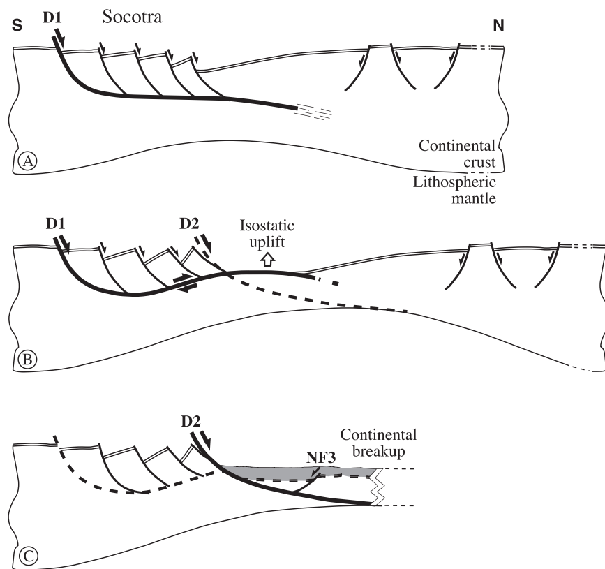
Figure 7. Conceptual model for the development of detachment faults onshore and offshore western Socotra (not to scale). (a) Stage 1: formation of the first detachment (D1). (b) Stage 2: isostatic uplift of the distal part of D1, which became inactive. (c) Stage 3: formation of the second detachment (D2) or low-angle normal fault. NF3: antithetic normal fault cutting D1.
