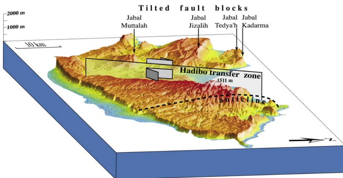
Figure 3. Segmentation of the continental margin by the Hadibo transfer zone illustrated by the SRTM digital elevation model of Socotra view from the east (N110°E). The broad asymmetric anticline of eastern Socotra in the foreground is separated from the four tilted blocks of western Socotra in the background by the right-lateral Hadibo transfer zone.
