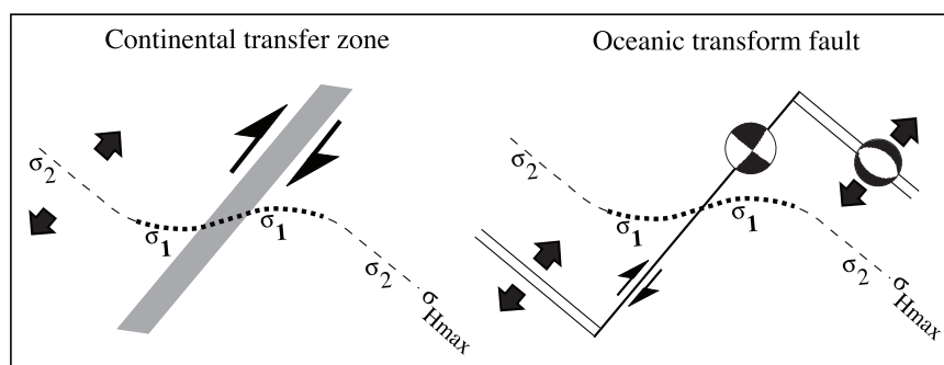
Figure 4. Comparison of maximum horizontal stress trajectories ( \sigma_{Hmax} ) for a right-lateral continental transfer zone and an oceanic transform fault. In the vicinity of the transfer zone or transform fault, \sigma_{Hmax} switches from \sigma_2 to \sigma_1 and its direction rotates counterclockwise.
