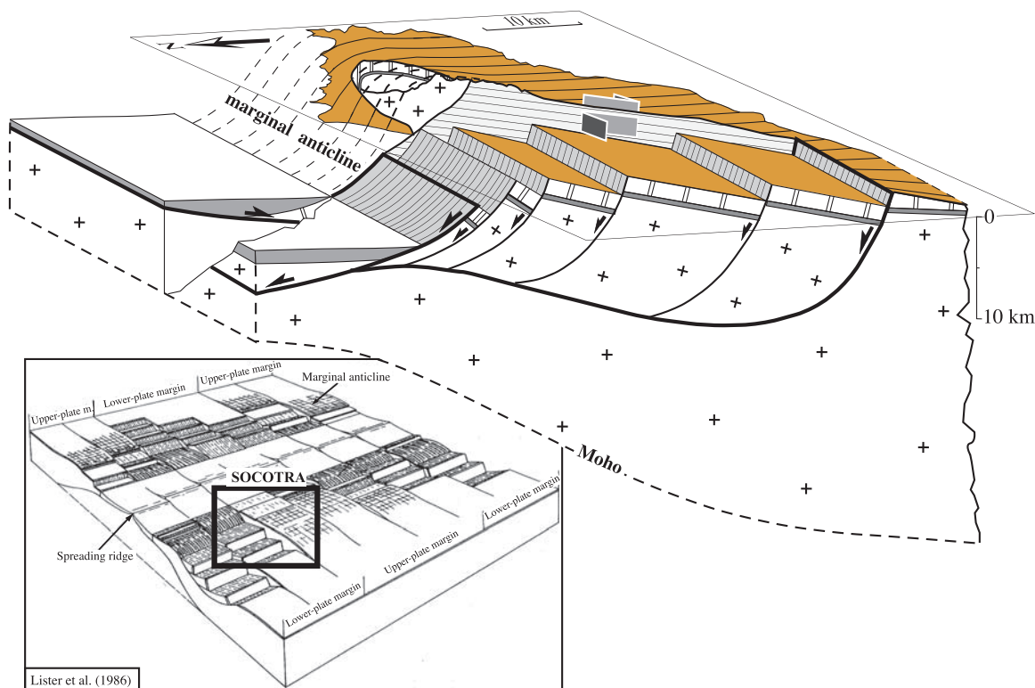
Figure 6. Along-strike change of sense of asymmetry of the southern margin of the Gulf of Aden on either side of the Hadibo transfer zone. It is proposed that the asymmetric structures of western and eastern Socotra are controlled at depth by detachment faults with opposite dips and senses of shear. The normal faults of western Socotra would sole out into a detachment surface with a top-to-the-north sense of shear, whereas the asymmetric anticline of eastern Socotra would be associated with a southward flattening detachment fault with a top-to-the-south sense of shear. Inset shows the detachment model of passive margins of Lister et al. [1986] with the possible location of Socotra.
