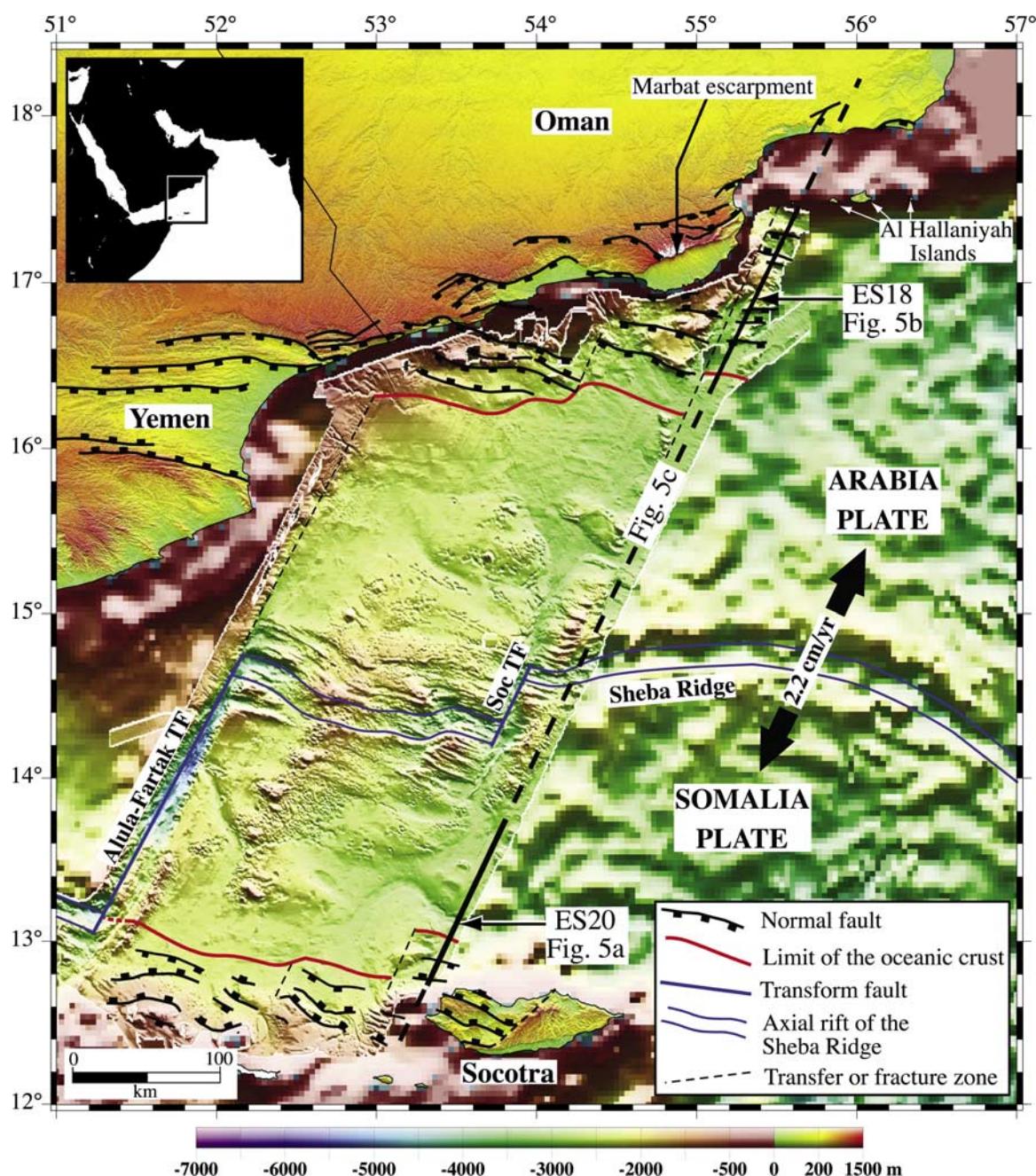
Figure 1. Geodynamical setting of the eastern Gulf of Aden and Socotra Island. Topography and bathymetry compiled from SRTM data onland [Farr and Kobrick, 2000] and multibeam soundings bathymetry from Encens-Sheba cruise [Leroy et al., 2004] superimposed on the world bathymetric map of Sandwell and Smith [1997] in the oceanic domain. Black arrows show plate relative motions [Fournier et al., 2001]. The dashed line shows location of the margin to margin cross section of Figure 5, and solid portions correspond to seismic reflection profiles ES18 and ES20 acquired during the Encens-Sheba cruise. Soc is Socotra. TF is transform fault.
