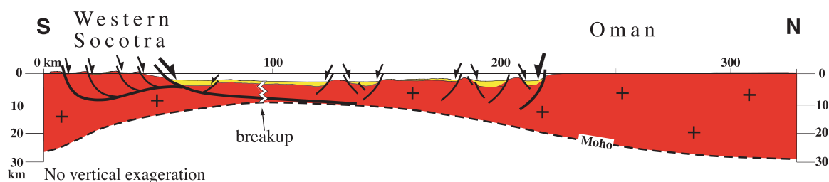
Figure 8. Prebreakup reconstruction of the eastern Gulf of Aden rift showing the complementary asymmetry of the opposing margins. The location of the breakup is offset toward the Socotra margin.
