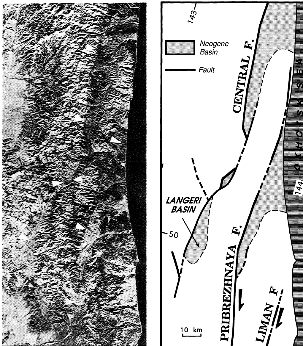
Fig. 16. Detail of the Landsat image of the East Sakhalin Mountains showing three parallel faults bounding Neogene basins.
