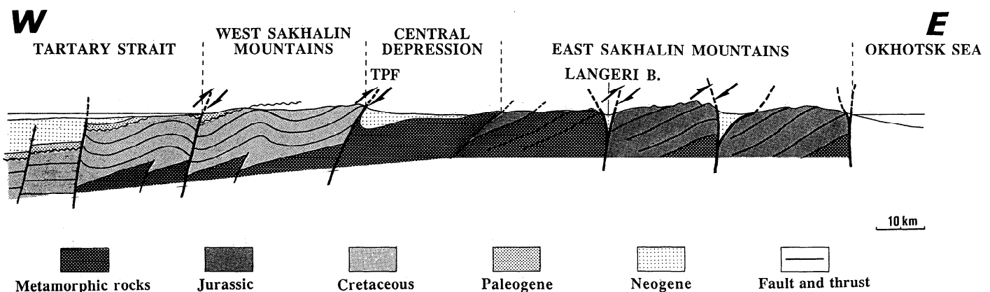
Fig. 5. East-west cross section of Sakhalin, localized in Figure 3c. B is basin, TPF is Tym-Poronaysk fault.
