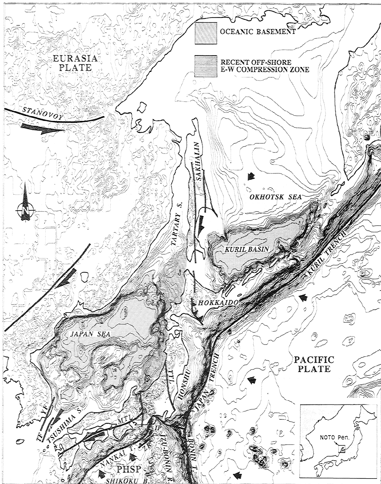
Fig. 1. Simplified structural map of far east Asia with topography and bathymetry. Solid arrows give directions of motions of Pacific and Okhotsk plates relative to Asia. B is basin, IP is Izu Peninsula, MTL is median tectonic line, R is ridge, S is strait, T is trench, TF is Tsushima fault, TTL is Tanakura tectonic line, YF is Yangsan fault, and ZR is Zenisu ridge.
