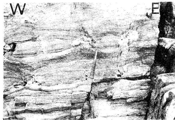
Fig. 8. Boudins of mafic sandstones metamorphosed into quartzites in the Oletta-Serra di Pigno cover (near Monte a a Torra, section b, Figure 3).
