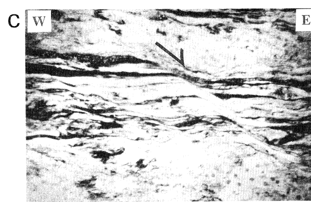
Fig. 13. Microscopic eastward shear criteria. (a) late albite crystallizing in asymmetric pressure shadows around garnet in the Lancône glaucophanites; (b) late albite crystal overprinting the earlier HP-BT foliation cut by eastward shear plane; (c) shear planes in the Cap Corse calcschist.
