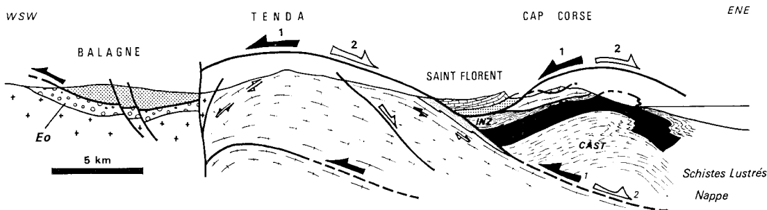
Fig. 2. Synthetic E-W cross section of the Cap Corse in the Bastia area [after Jolivet et al., 1990] (see location of the cross section in Figure 1). Solid arrows indicate the early westward compressional event (HP-LT); open arrows indicate the late eastward extensional event. For abbreviations see Figure 1. EO is Eocene autochthonous sediments.
