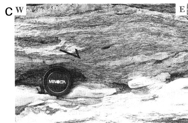
Fig. 12. Eastward shear criteria superposed along the main early thrust contacts. (a and b) Shear planes in the Paleozoic cover of the Tenda massif (west coast of the Saint-Florent gulf); (c) eastward shear plane in the Oletta-Serra di Pigno cover very near the contact with the gneisses.
