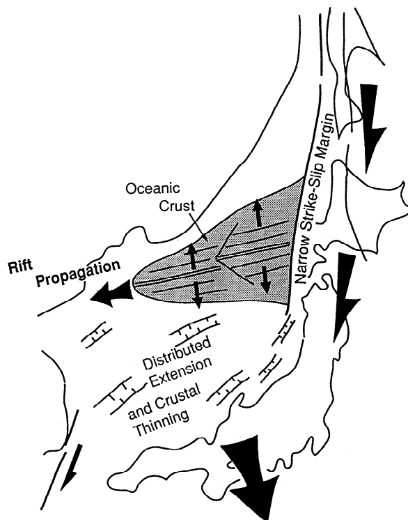
Figure 4. Simplified geometry of the Japan Sea opening after Jolivet and Tamaki [1992]. Distributed extension and oceanic spreading with westward propagation accommodate the southward motion of Japan along two major shear zones.
