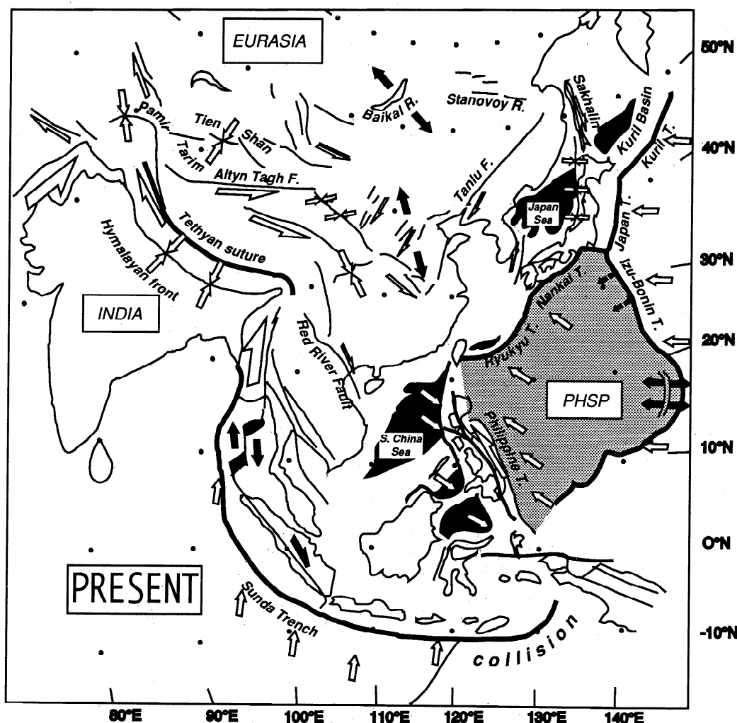
Figure 1. General geodynamic framework of Asia, Southeast Asia, and the northwest Pacific. Fault pattern inside Asia after Tapponnier et al. [1982]. Double open arrows represent the direction of relative convergence across intracontinental thrust zones, open semi-arrows represent the sense of relative motion along major strike-slip faults, open single arrows represent relative direction of motion of the subducting plate in subduction zones, and solid divergent arrows represent direction of relative divergence across major zones of extension.
