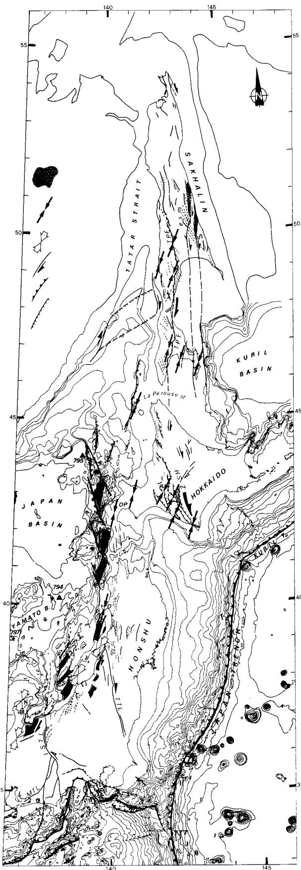
Fig. 2. Tectonic map of the entire shear zone: 1, oceanic crust; 2, en échelon extensional basins of Miocene age; 3, direction of Miocene maximum compression deduced from fault set analysis; 4, sameas for 3 but intermediate compression; 6, strike-slip faults; 7, thrust faults; and 8, normal faults. Abbreviations are esm, East Sakhalin Moutains; OP, Oshima peninsula; O, Oga peninsula; N, Noto peninsula; IZU, Izu peninsula, TPF, Tym-Poronaik Fault; MTL, Median Tectonic Line; TTL, Tanakura Tectonic Line; ISTL, Itoigawa-Shizuoka Tectonic Line; HSZ, Hidaka Shear Zone, and TTT: trench-trench-trench triple junction of Central Japan.
