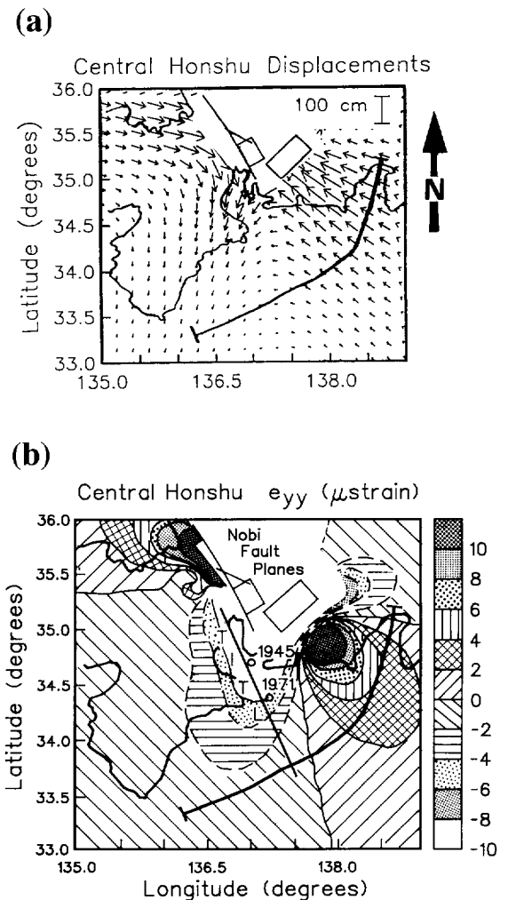
Fig. 4. Geographical pattern for (a) vector displacement and (b) strain release e_{yy} due to the 1891 Nobi earthquake (defined as the coseismic + post-seismic strain release calculated at the boundary of complete relaxation). The y-axis is taken to be the direction N40^\circ W . The heavy line represents the axis of the Nankai trough. Four rectangular fault planes (two vertical and two dipping fault planes) used to model the Nobi fault ruptures [41] are shown for reference. In (b), positive/negative values correspond to an increase in tension/compression. The epicentres of the M = 7.1 1945 Mikawa and M = 6.1 1971 Atumi–Oki earthquakes [55] and the oceanward extension of the Tsuruga Bay–Ise bay Tectonic Line are superimposed. Modified from [25].
