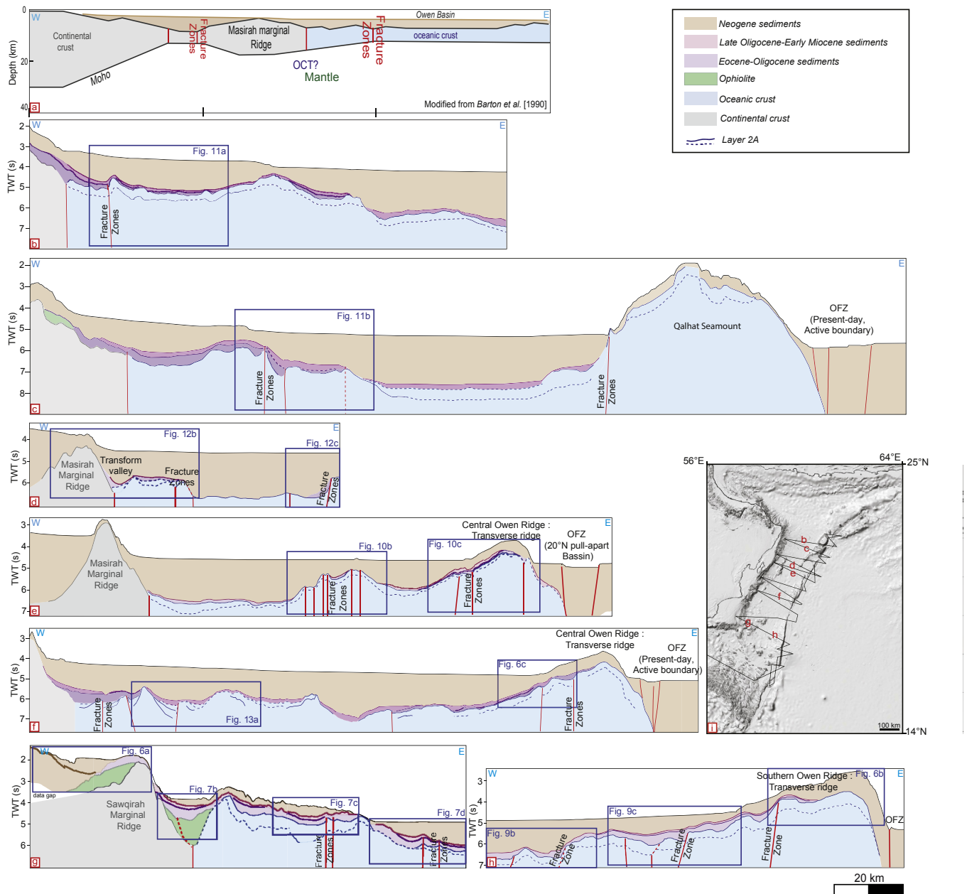
Fig. 5. a) Deep-structure of the Owen Basin deduced from wide-angle seismic data (Barton et al., 1990), see Fig. 3a for location. OCT: inferred ocean-continent transition. b) to h): Simplified picking of large scale seismic profiles, and locations of close-views of seismic profiles displayed hereafter. i) Location of seismic profiles, same as Fig. 3.
